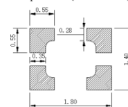
Land pattern (Recommended)
