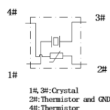
Terminal land connections
